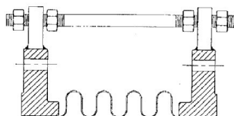
Limiting Rod detail
